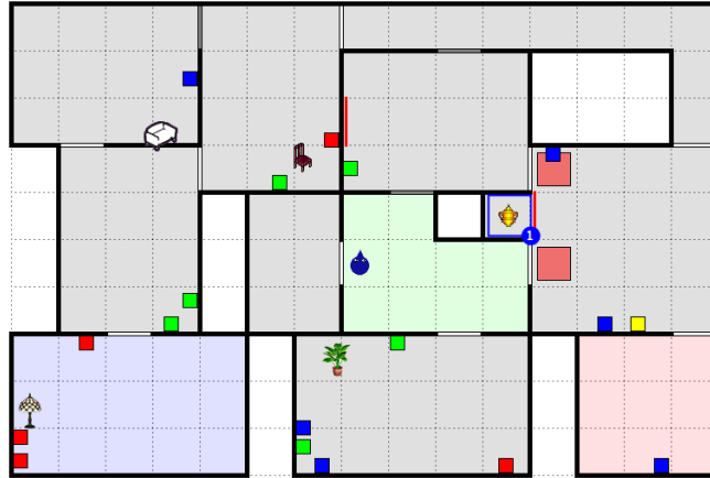
Figure 3: Virtual world 1.
