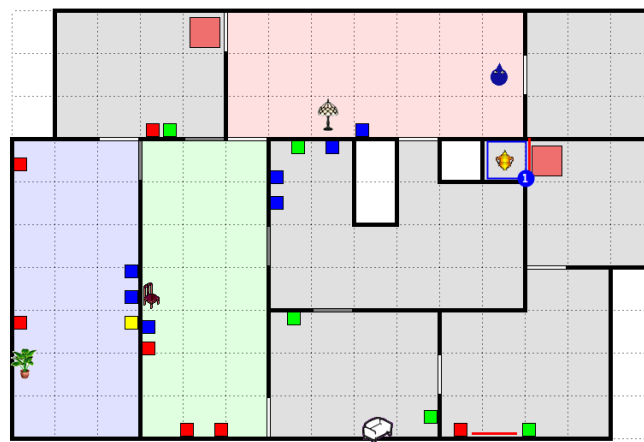
Figure 4: Virtual world 2.
