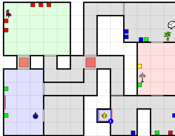
Figure 5: Virtual world 3.
