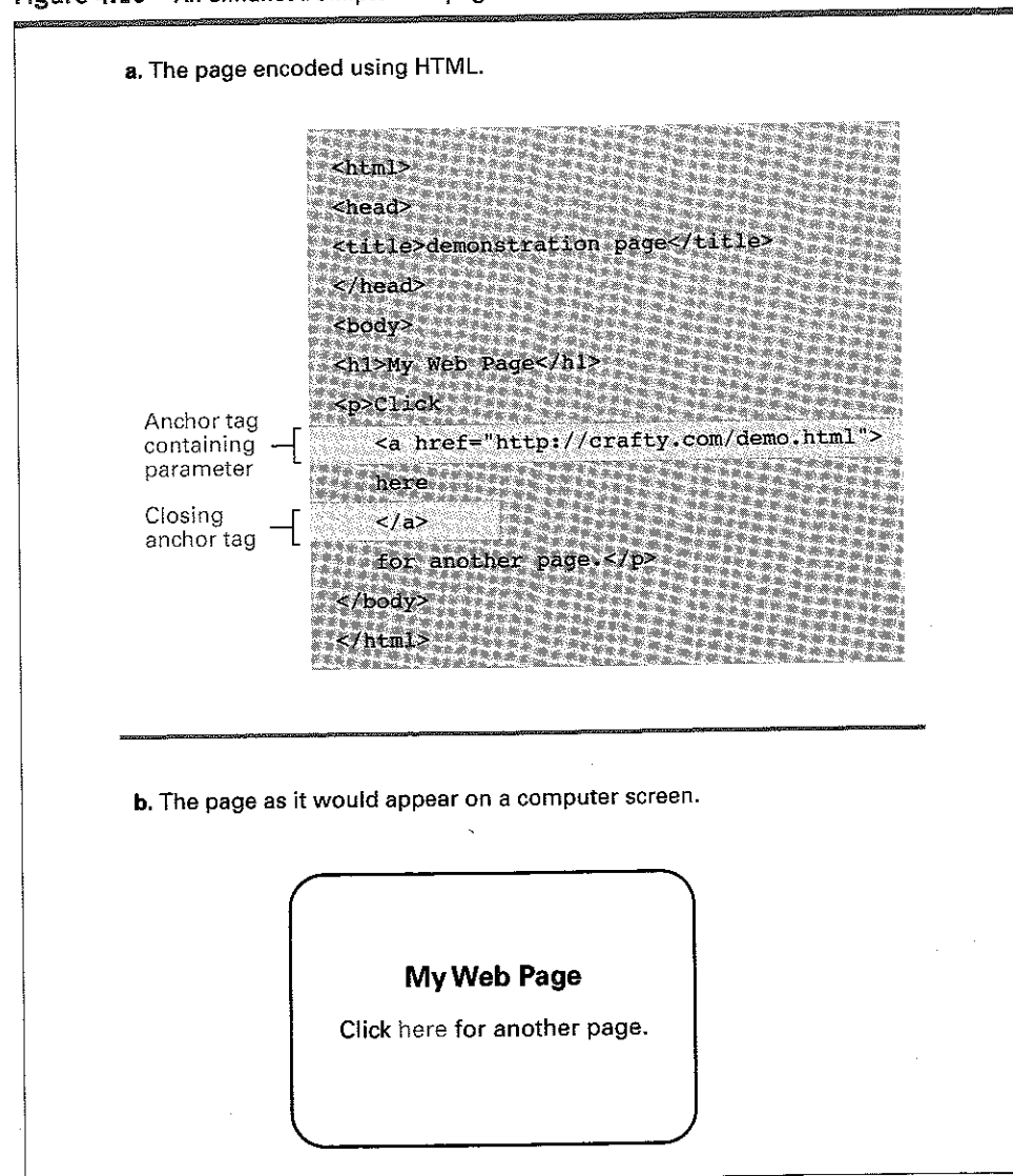
Figure 4.10 An enhanced simple Web page
