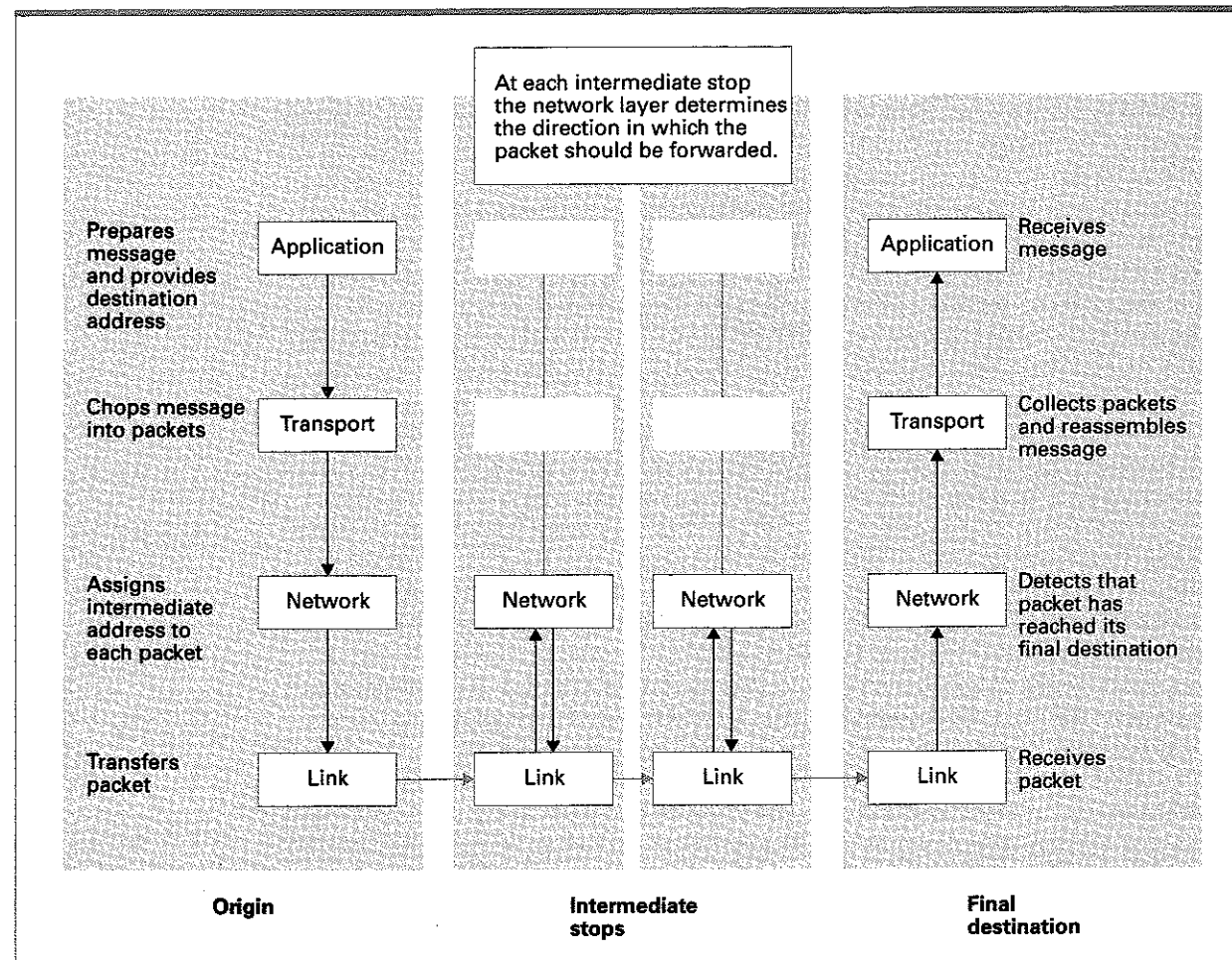
Figure 4.14 Following a message through the Internet
